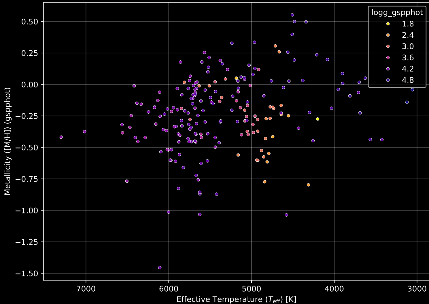
APOGEE DR17 Field: [102+59_MGA] Stellar Population Parameters (n= 206)
