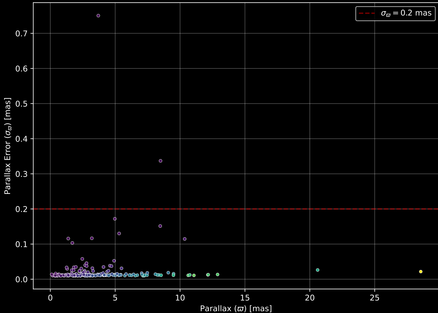
APOGEE DR17 Field: [102+59_MGA] Parallax Quality (n= 206)
