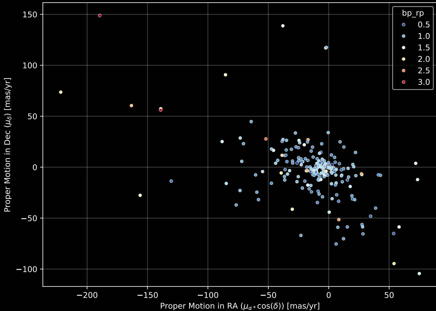
APOGEE DR17 Field: [102+59_MGA] Proper Motion Diagram (n= 206)
