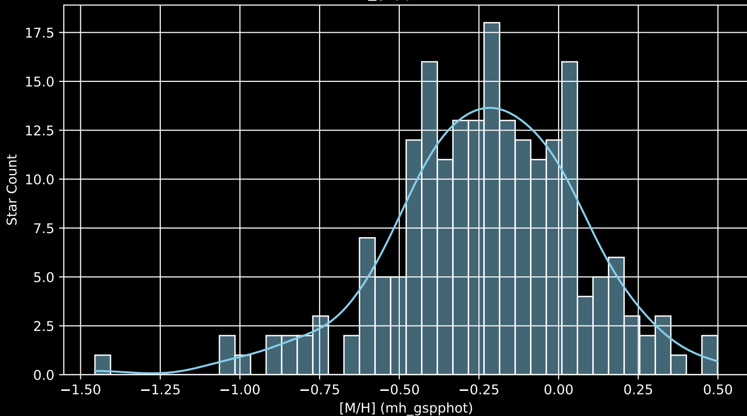
APOGEE DR17 Field: [102+59_MGA [M/H] (mh_gspphot) (n= 205)
