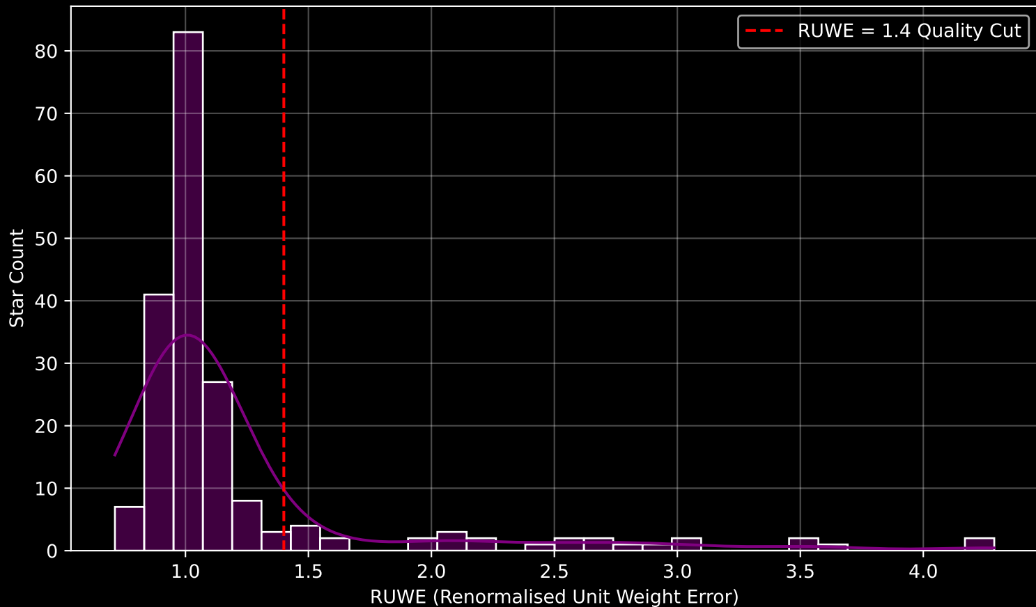
GAPOGEE DR17 Field [102+59_MGA] RUWE Distribution (n= 196)
