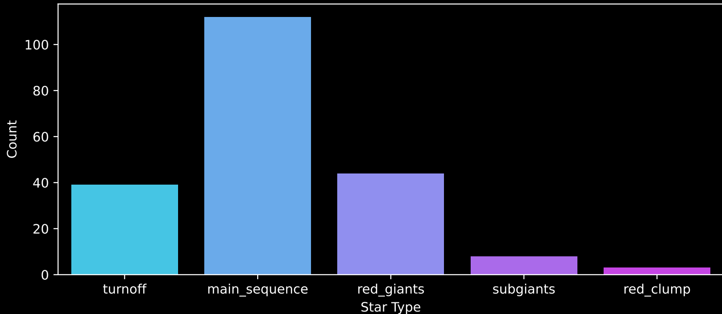
APOGEE DR17 Field: [102+59_MGA] Count plot of Star Type
